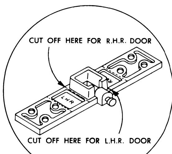
TOP BOLT GUIDE ASSEMBLY FIG. 2B
