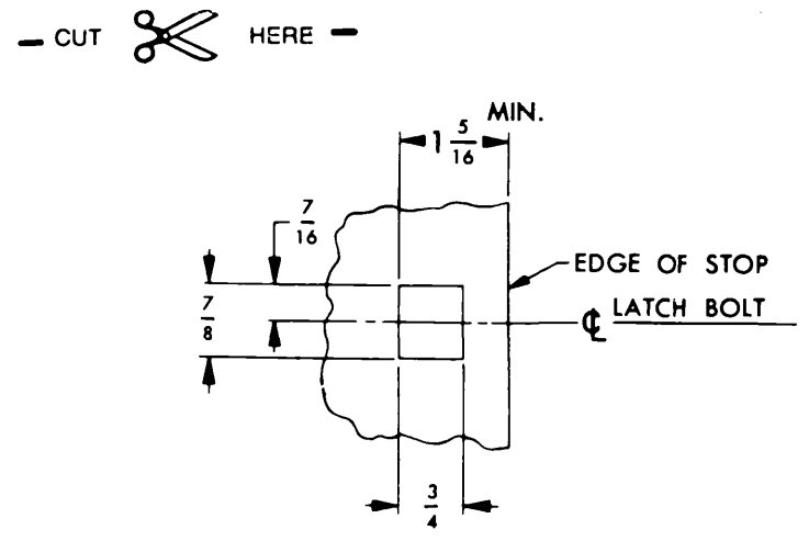
REINFORCED HOLLOW METAL AND ALUMINUM FRAME PREPARATION FIG. 9C
