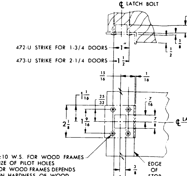
WOOD FRAME PREPARATION FIG. 9A
